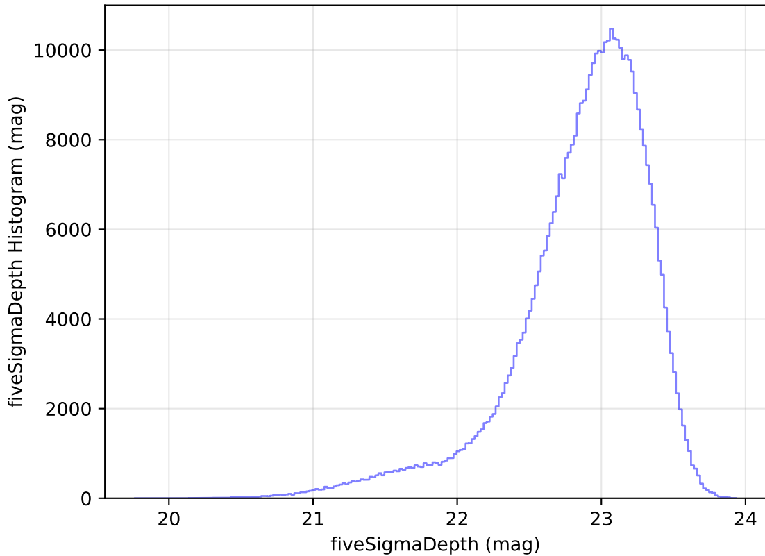
weather_cloudso4v3.4_10yrs All sky z band: fiveSigmaDepth Histogram
