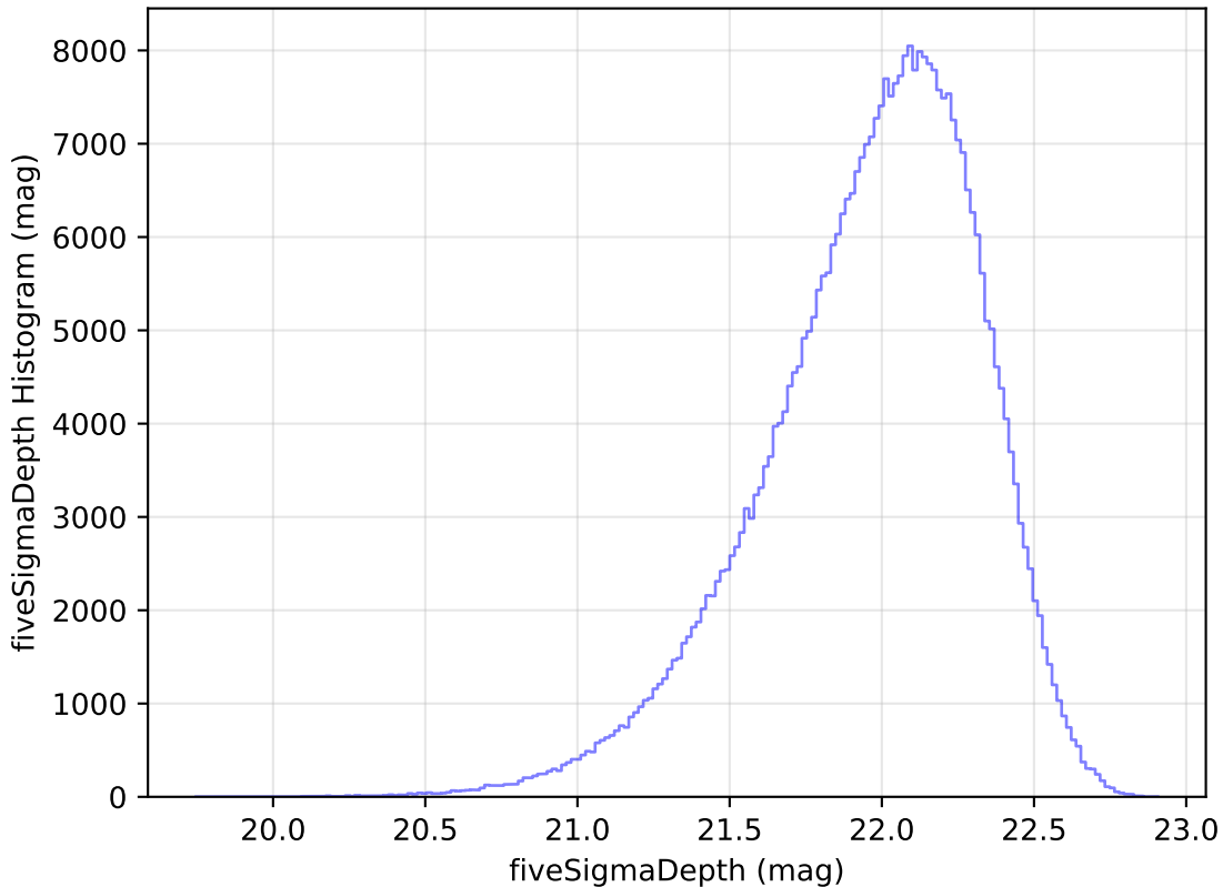
weather_cloudso4v3.4_10yrs All sky y band: fiveSigmaDepth Histogram
