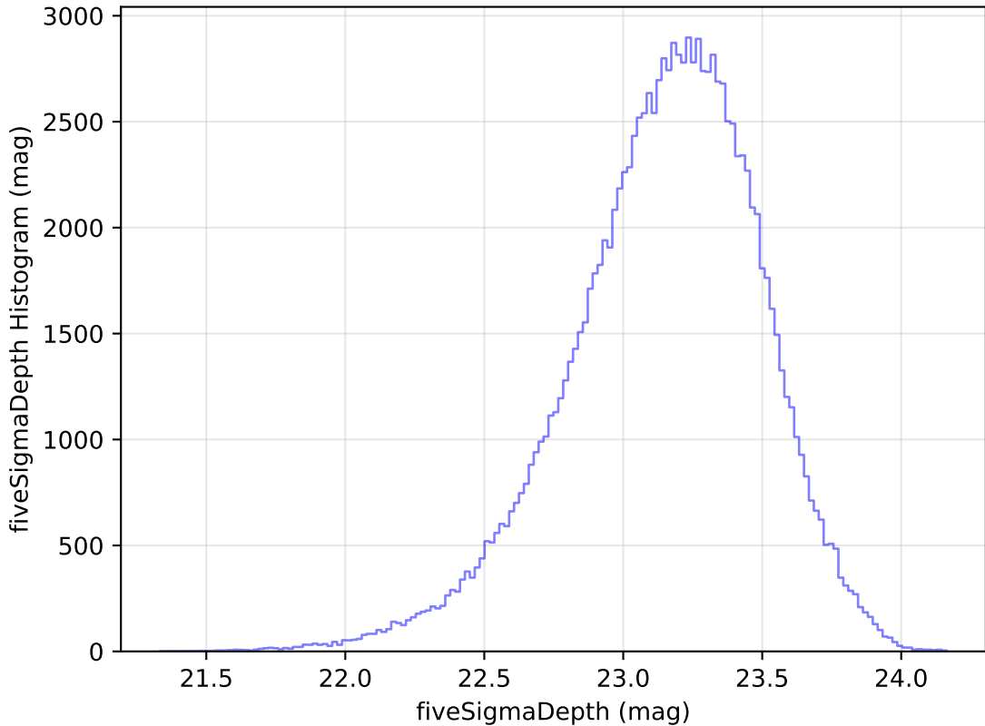
weather_cloudso4v3.4_10yrs All sky u band: fiveSigmaDepth Histogram
