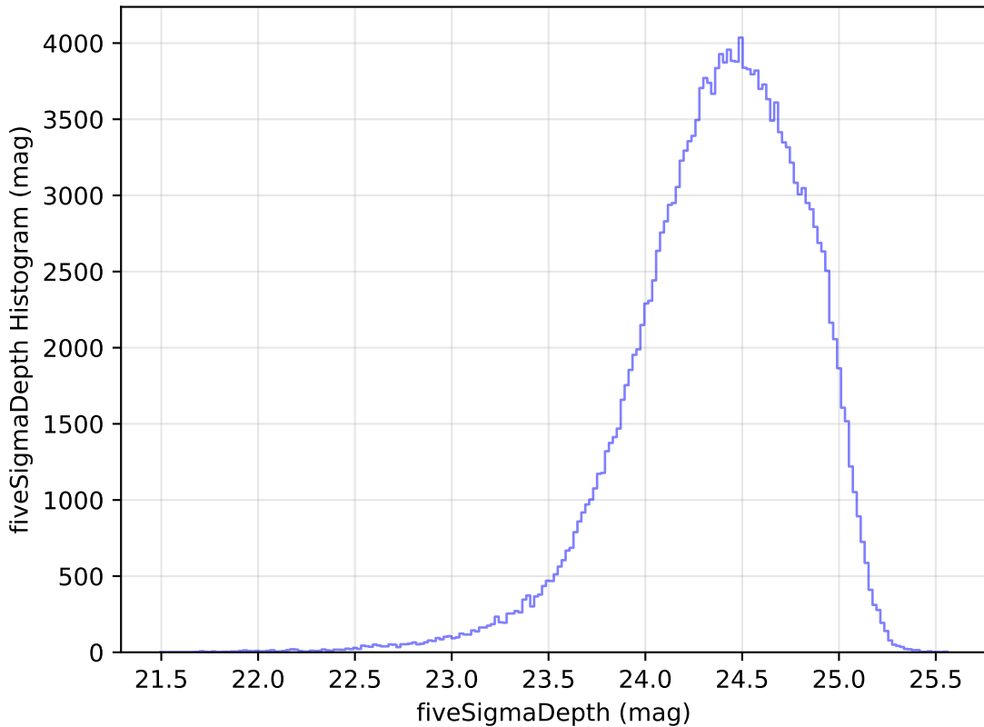
weather_cloudso4v3.4_10yrs All sky g band: fiveSigmaDepth Histogram
