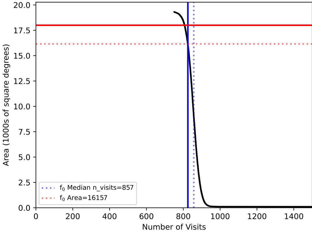
weather_cloudso4v3.4_10yrs WFD: f0
