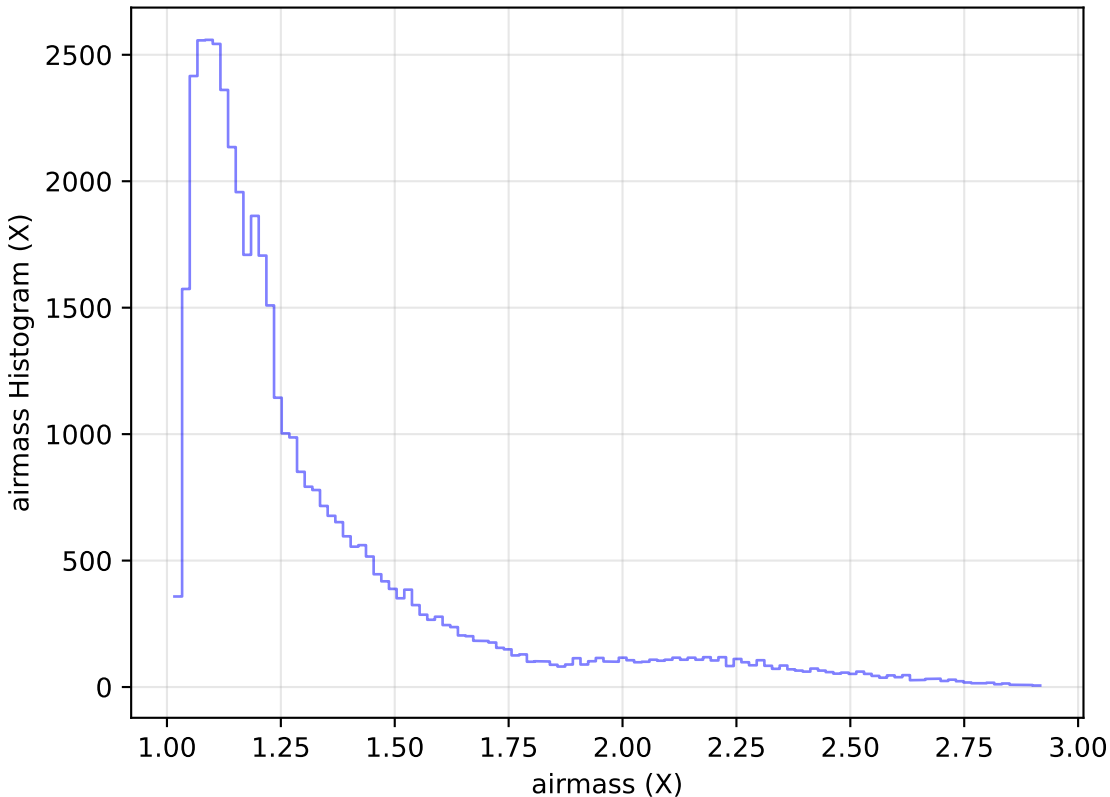
weather_cloudso4v3.4_10yrs Yr 1 z band: airmass Histogram
