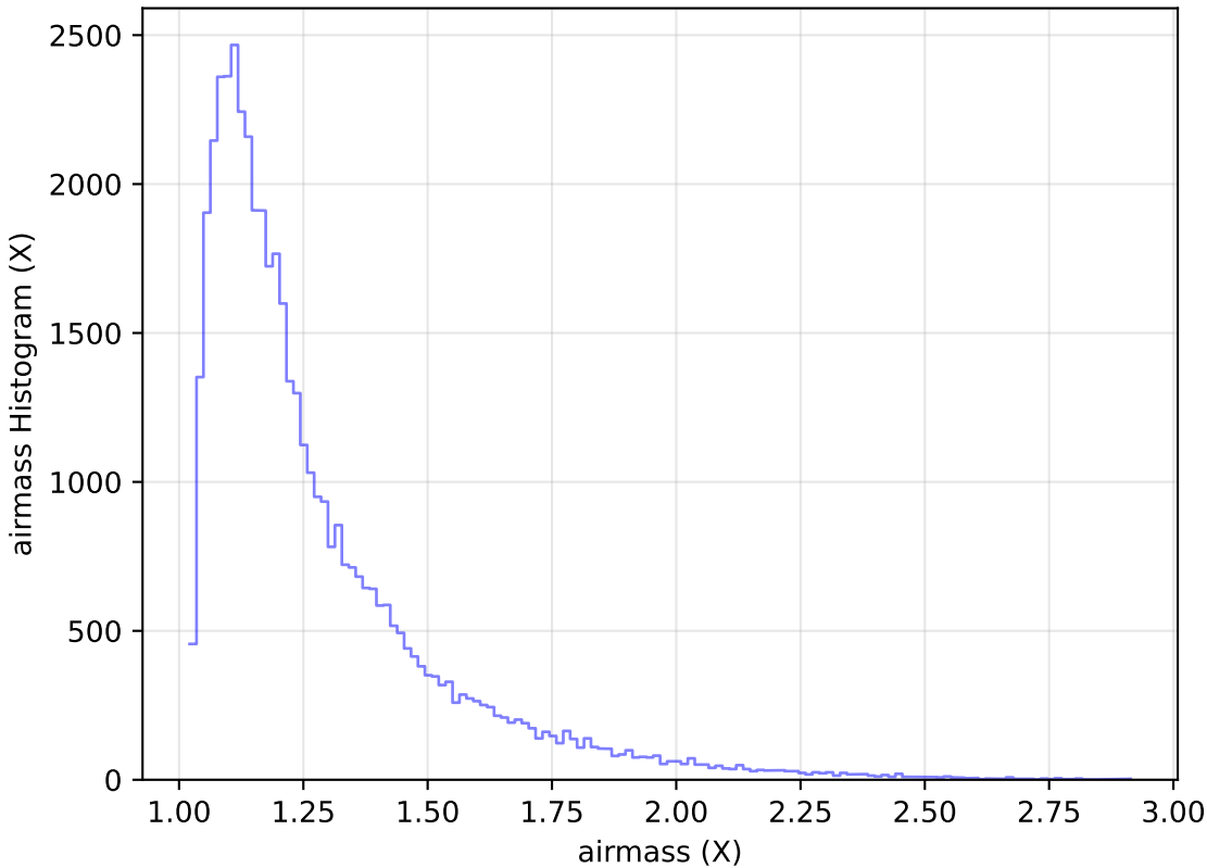
weather_cloudso4v3.4_10yrs Yr 1 y band: airmass Histogram
