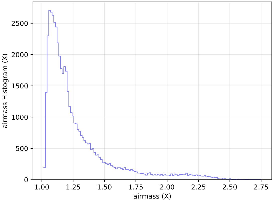
weather_cloudso4v3.4_10yrs Yr 1 r band: airmass Histogram
