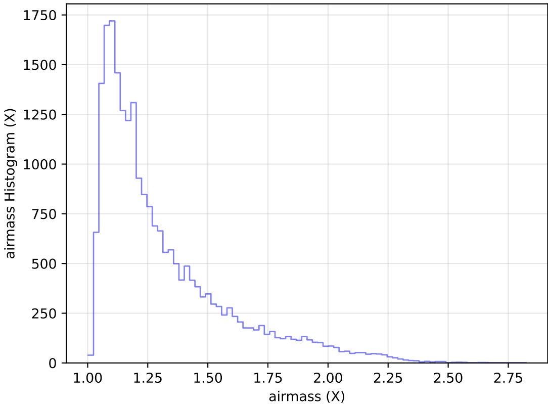
weather_cloudso4v3.4_10yrs Yr 1 g band: airmass Histogram
