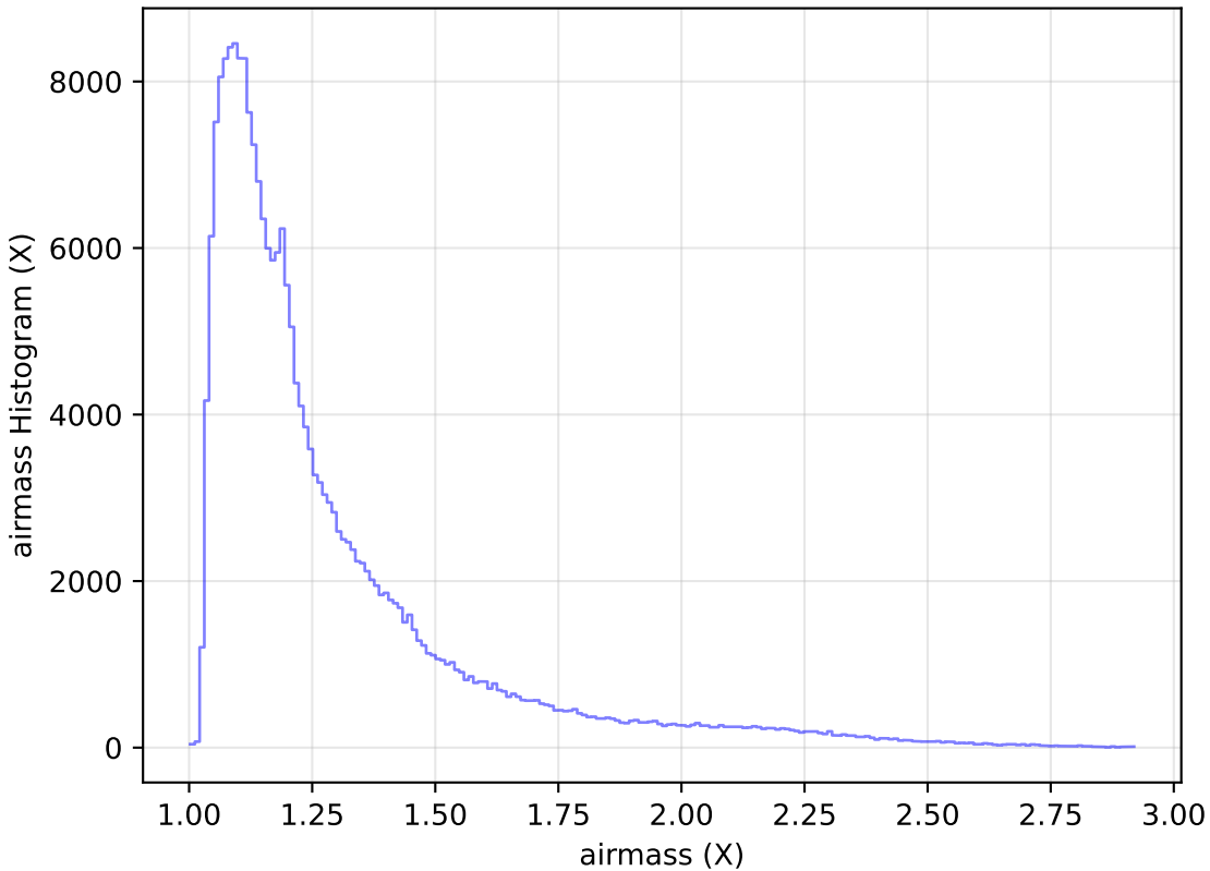
weather_cloudso4v3.4_10yrs Yr 1 all bands: airmass Histogram
