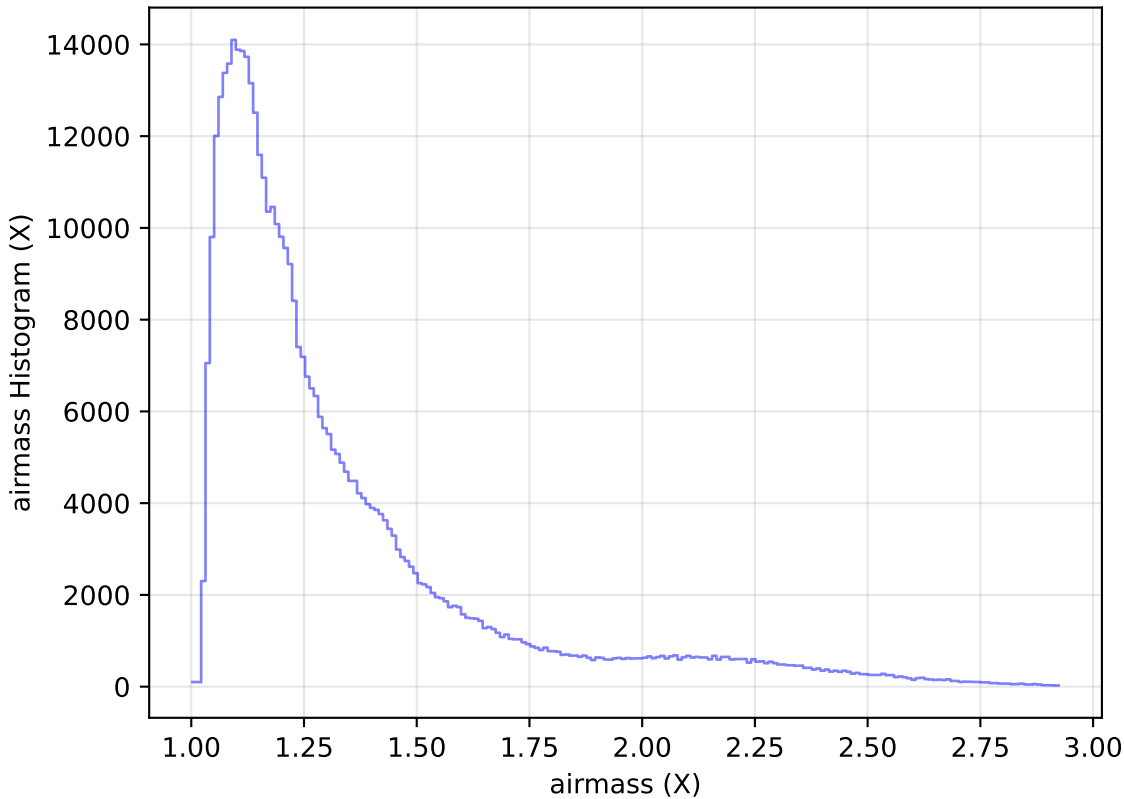
weather_cloudso4v3.4_10yrs WFD z band: airmass Histogram
