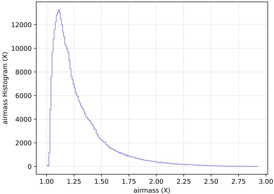
weather_cloudso4v3.4_10yrs WFD y band: airmass Histogram
