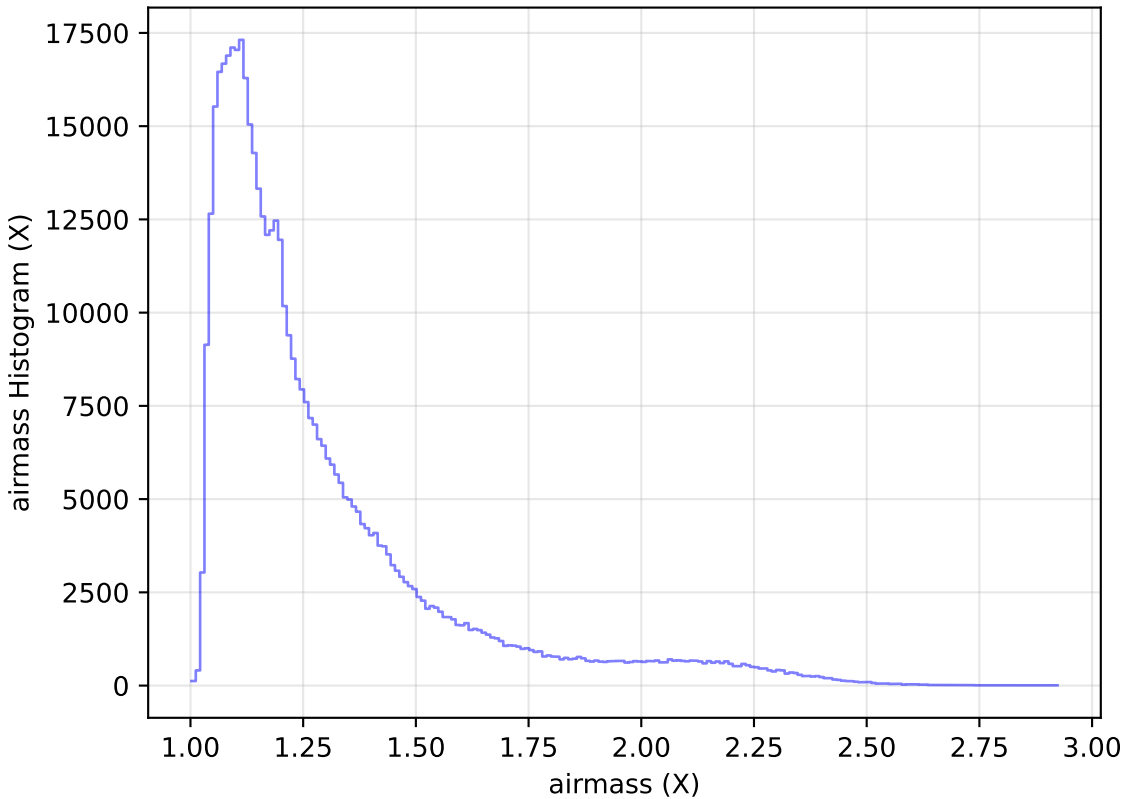
weather_cloudso4v3.4_10yrs WFD r band: airmass Histogram
