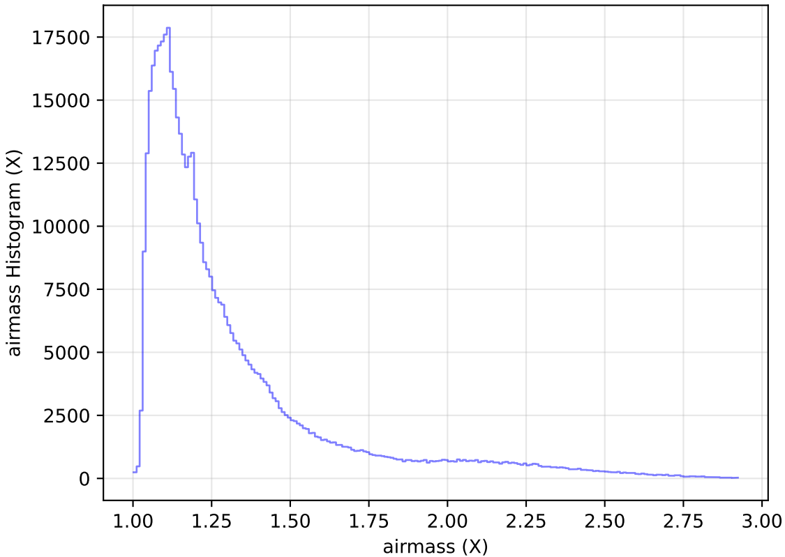
weather_cloudso4v3.4_10yrs WFD i band: airmass Histogram
