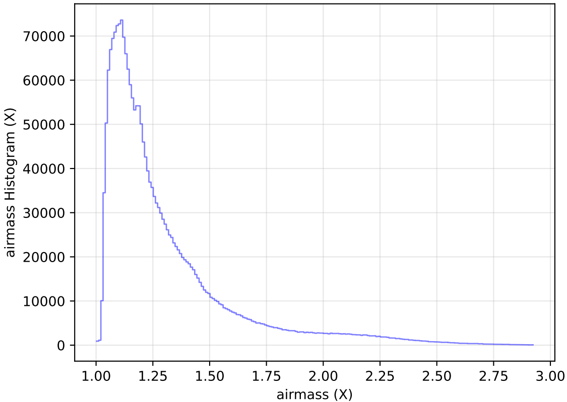
weather_cloudso4v3.4_10yrs WFD all bands: airmass Histogram
