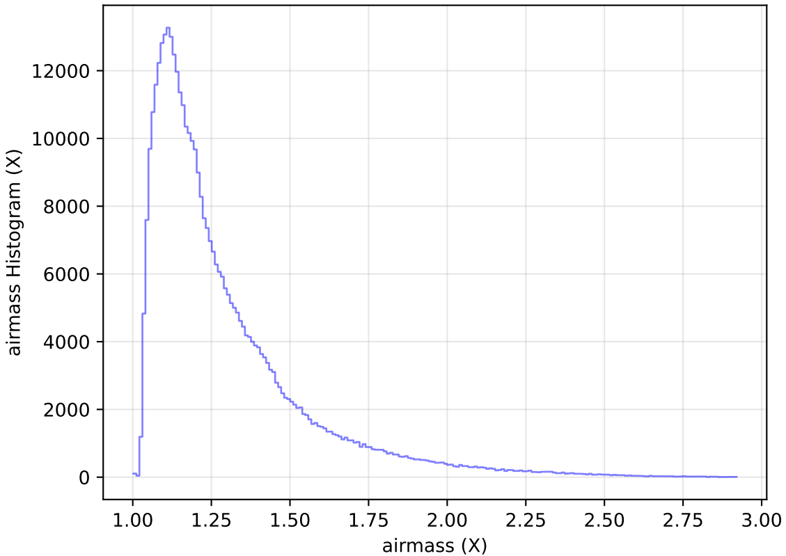
weather_cloudso4v3.4_10yrs All sky y band: airmass Histogram
