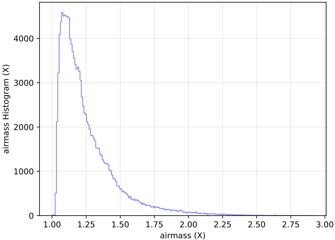
weather_cloudso4v3.4_10yrs All sky u band: airmass Histogram
