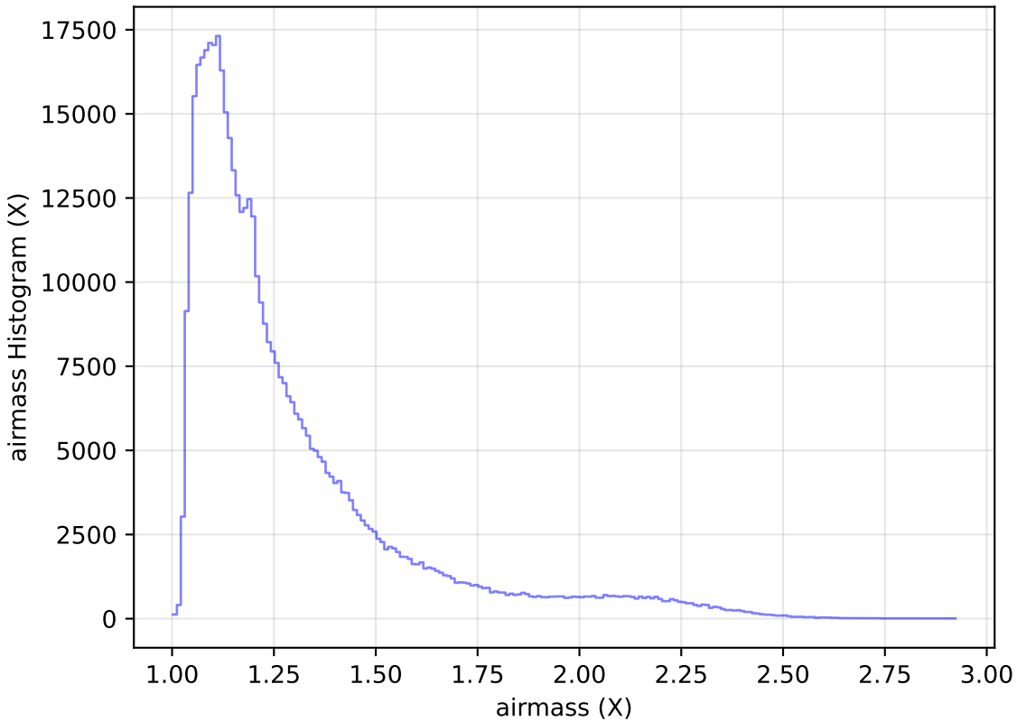
weather_cloudso4v3.4_10yrs All sky r band: airmass Histogram
