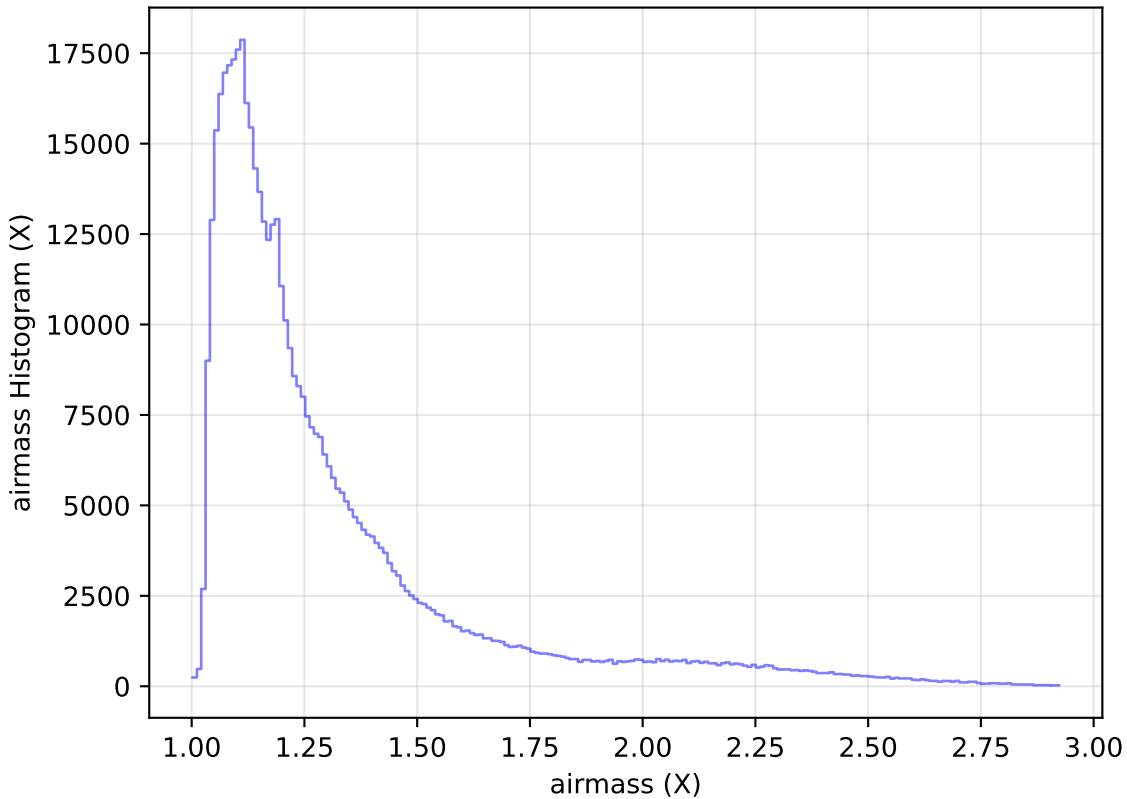
weather_cloudso4v3.4_10yrs All sky i band: airmass Histogram
