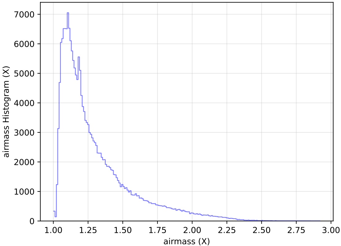
weather_cloudso4v3.4_10yrs All sky g band: airmass Histogram
