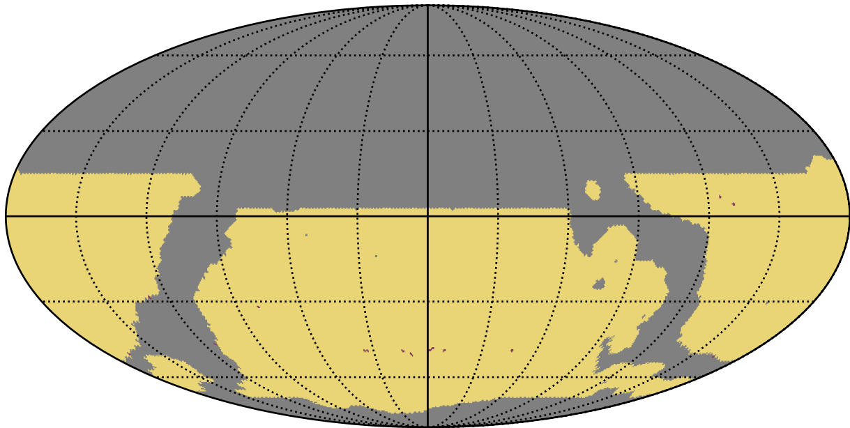
weather_cloudso4v3.4_10yrs WFD: RapidRevisits
