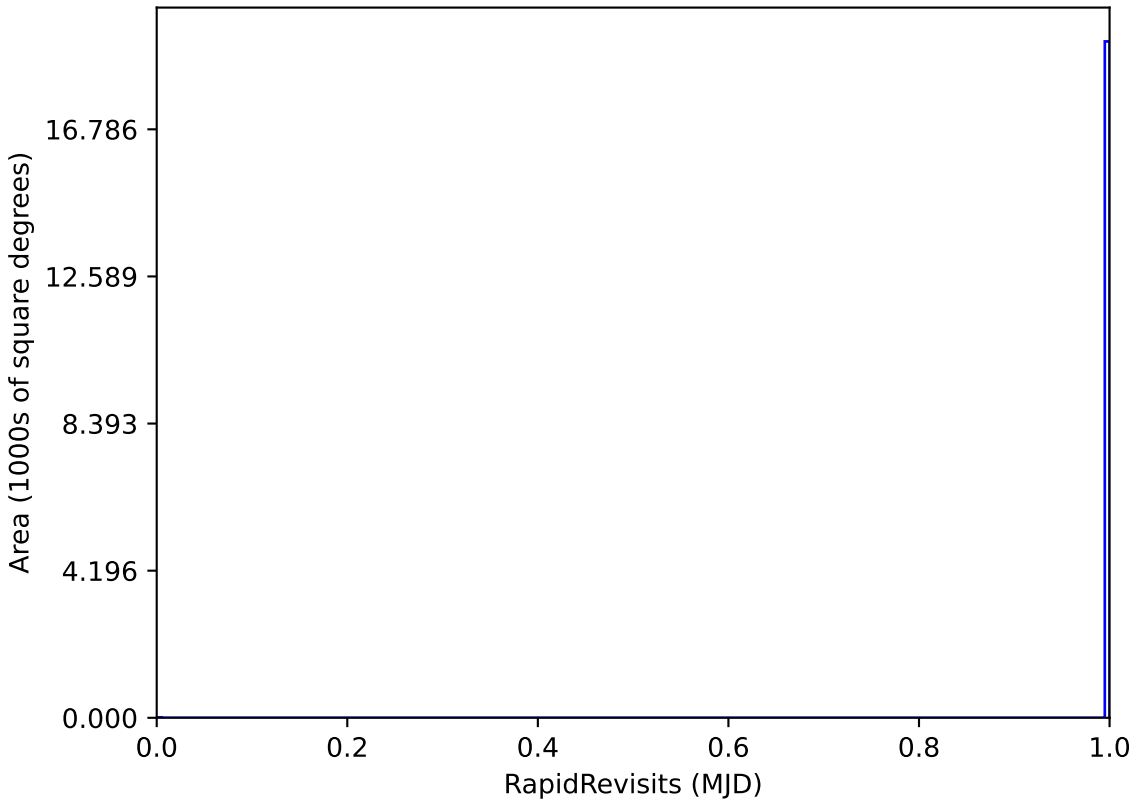
weather_cloudso4v3.4_10yrs WFD: RapidRevisits
