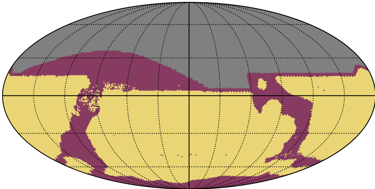
weather_cloudso4v3.4_10yrs All sky: RapidRevisits
