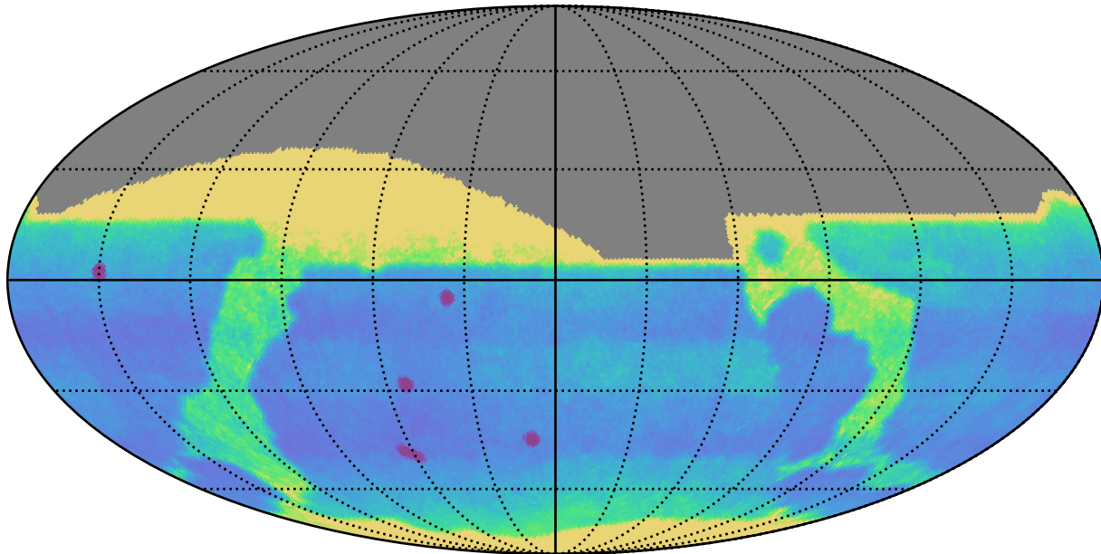
weather_cloudso4v3.4_10yrs All sky: Proper Motion Uncert @ 24.0
