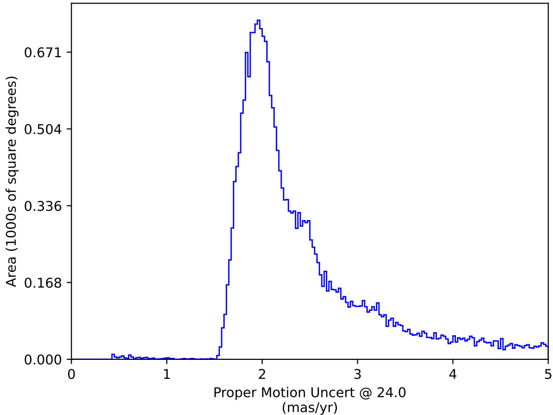
weather_cloudso4v3.4_10yrs All sky: Proper Motion Uncert @ 24.0
