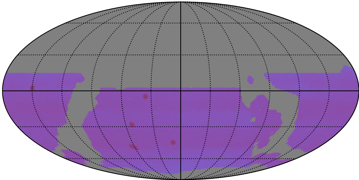
weather_cloudso4v3.4_10yrs WFD: Proper Motion Uncert @ 20.5
