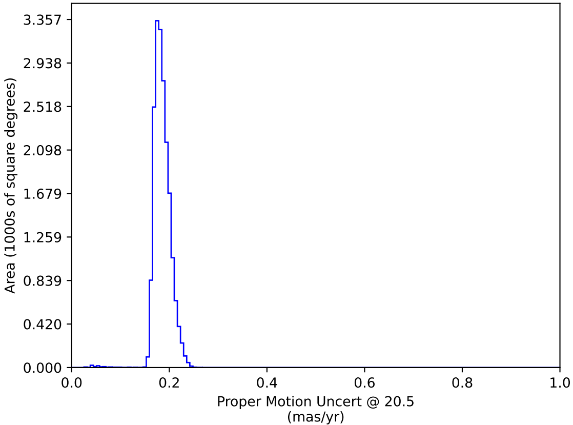
weather_cloudso4v3.4_10yrs WFD: Proper Motion Uncert @ 20.5
