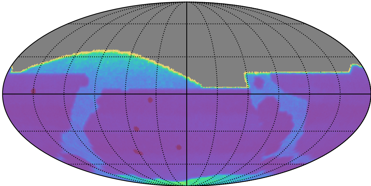
weather_cloudso4v3.4_10yrs All sky: Proper Motion Uncert @ 20.5
