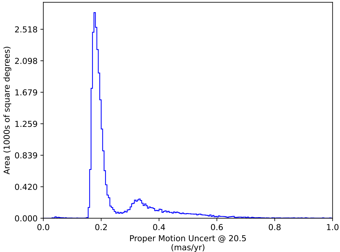
weather_cloudso4v3.4_10yrs All sky: Proper Motion Uncert @ 20.5
