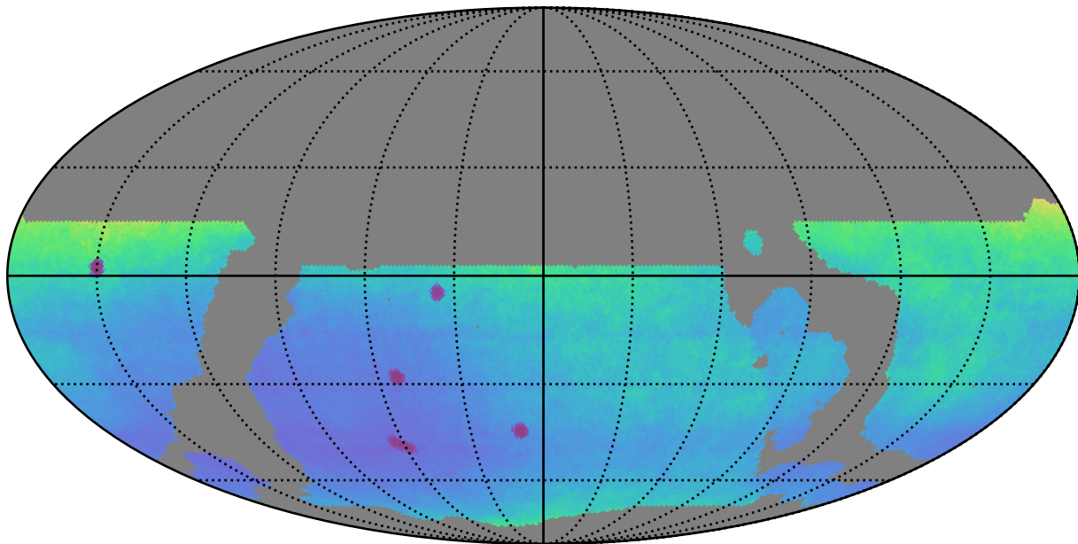
weather_cloudso4v3.4_10yrs WFD: Parallax Uncert @ 24.0
