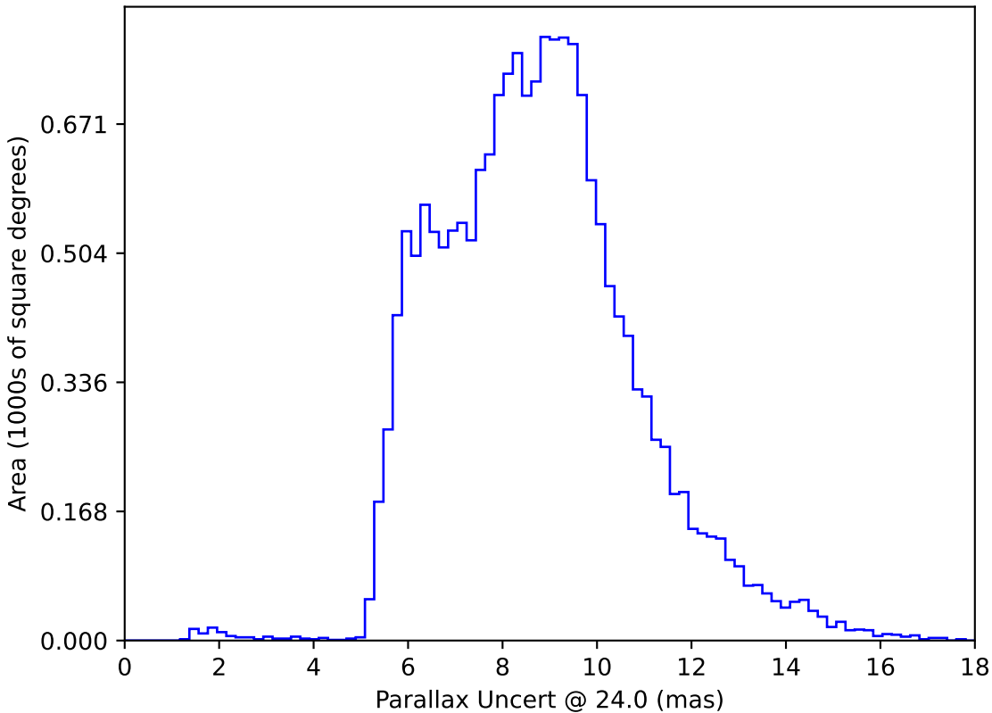
weather_cloudso4v3.4_10yrs WFD: Parallax Uncert @ 24.0
