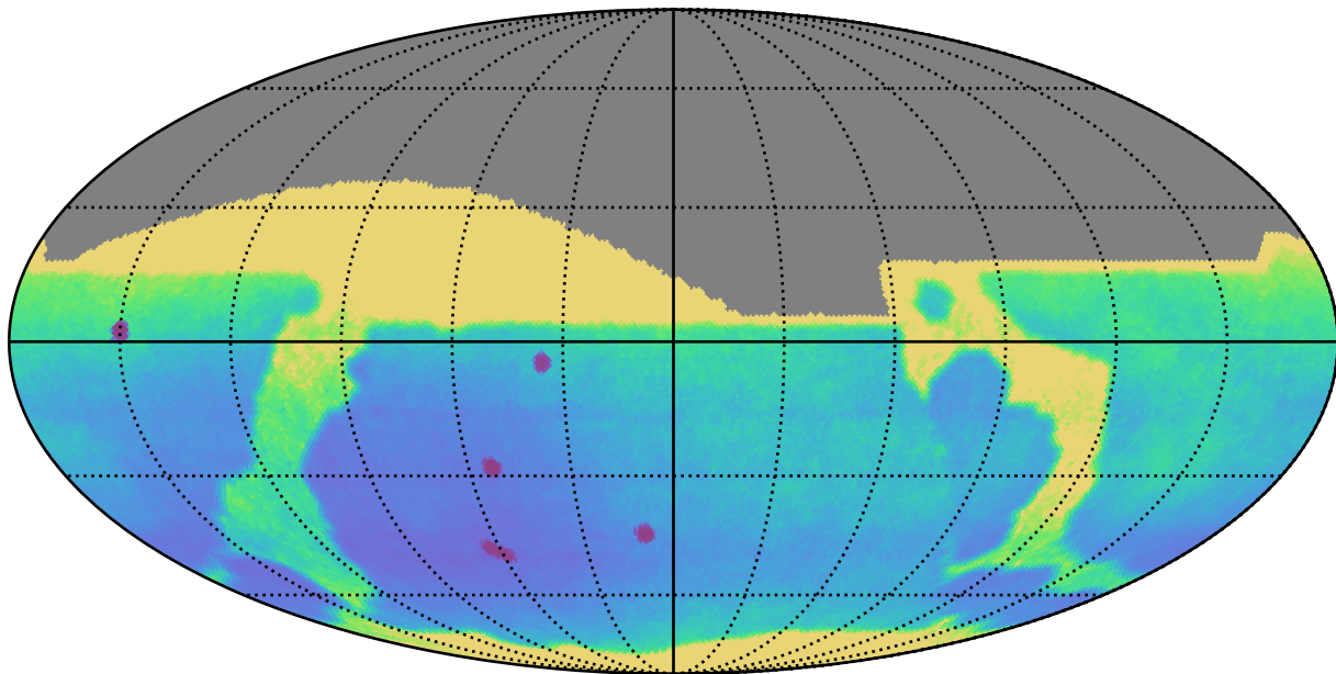
weather_cloudso4v3.4_10yrs All sky: Parallax Uncert @ 24.0
