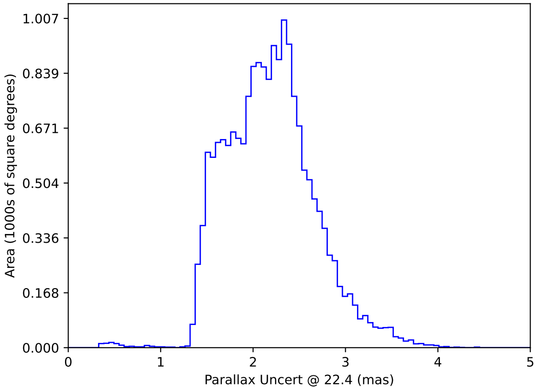
weather_cloudso4v3.4_10yrs WFD: Parallax Uncert @ 22.4
