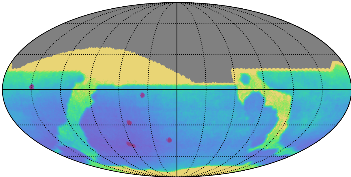
weather_cloudso4v3.4_10yrs All sky: Parallax Uncert @ 22.4
