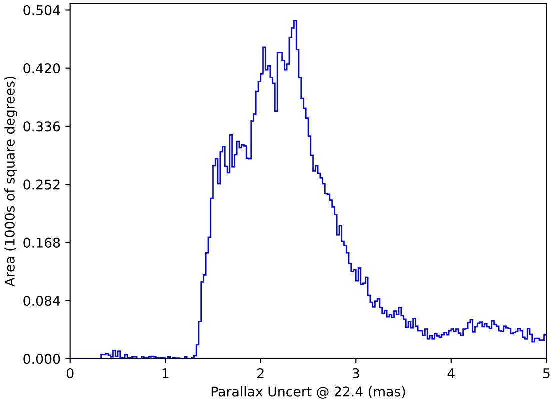
weather_cloudso4v3.4_10yrs All sky: Parallax Uncert @ 22.4
