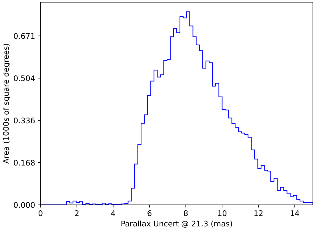
weather_cloudso4v3.4_10yrs WFD y band only: Parallax Uncert @ 21.3
