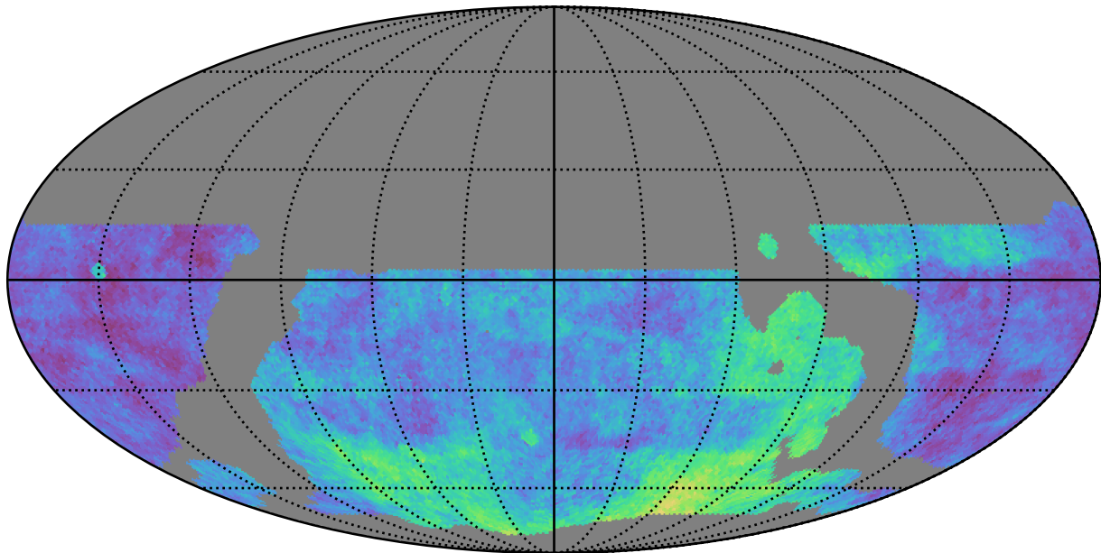
weather_cloudso4v3.4_10yrs WFD: Parallax Coverage @ 24.0
