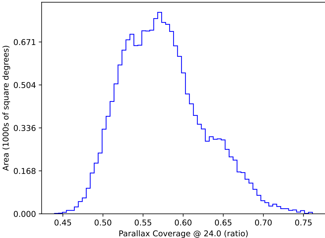
weather_cloudso4v3.4_10yrs WFD: Parallax Coverage @ 24.0
