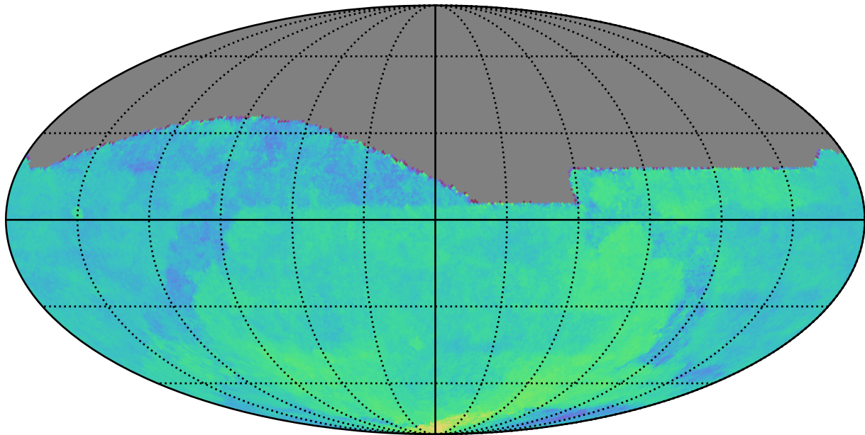
weather_cloudso4v3.4_10yrs All sky: Parallax Coverage @ 24.0
