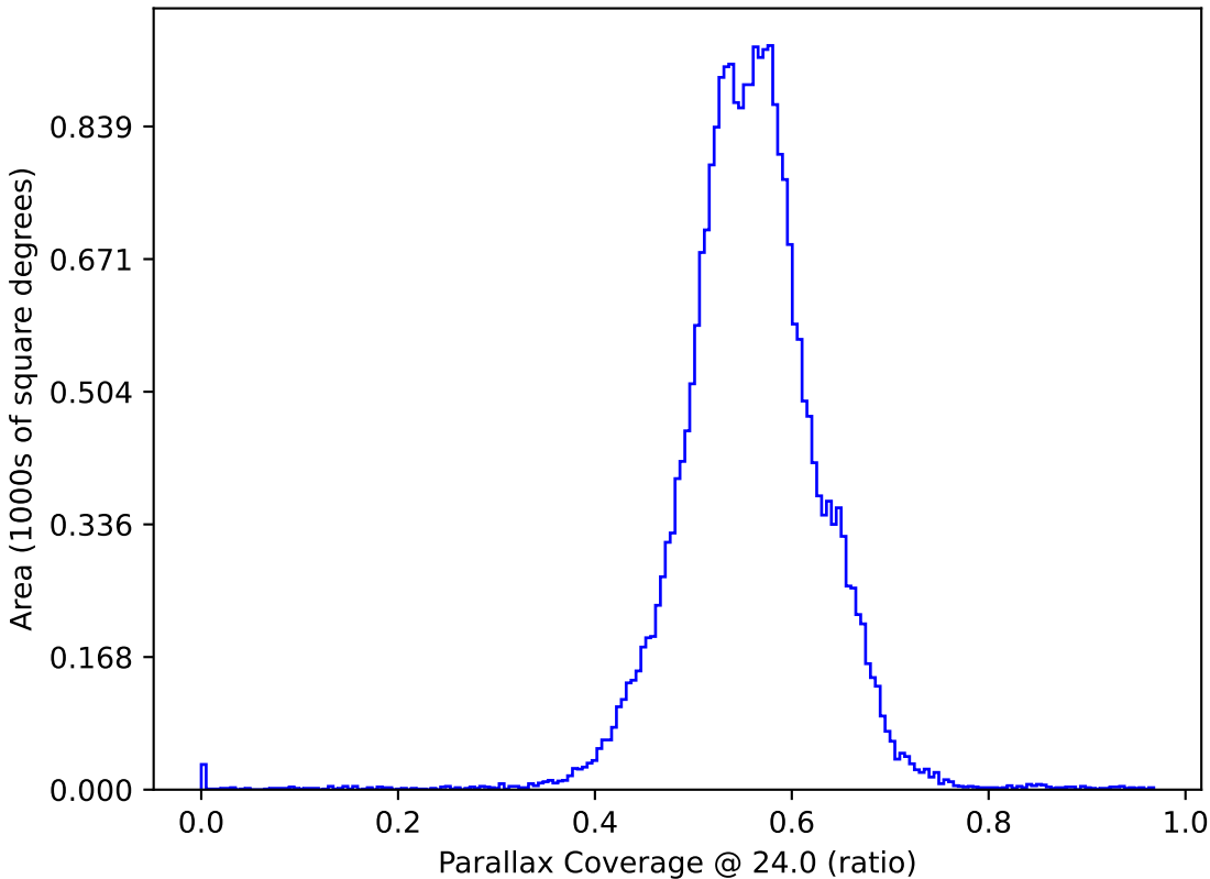
weather_cloudso4v3.4_10yrs All sky: Parallax Coverage @ 24.0
