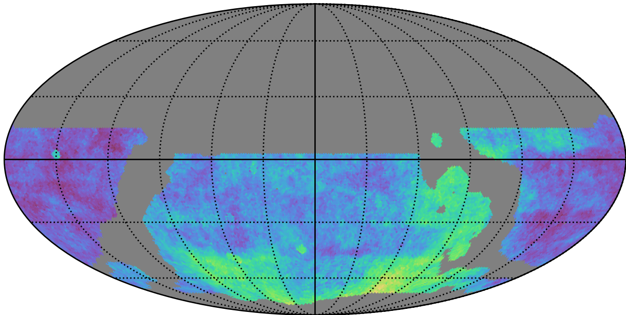
weather_cloudso4v3.4_10yrs WFD: Parallax Coverage @ 22.4
