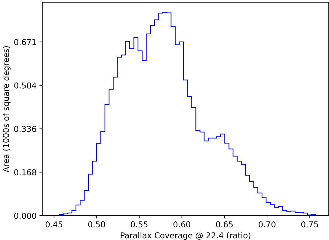
weather_cloudso4v3.4_10yrs WFD: Parallax Coverage @ 22.4
