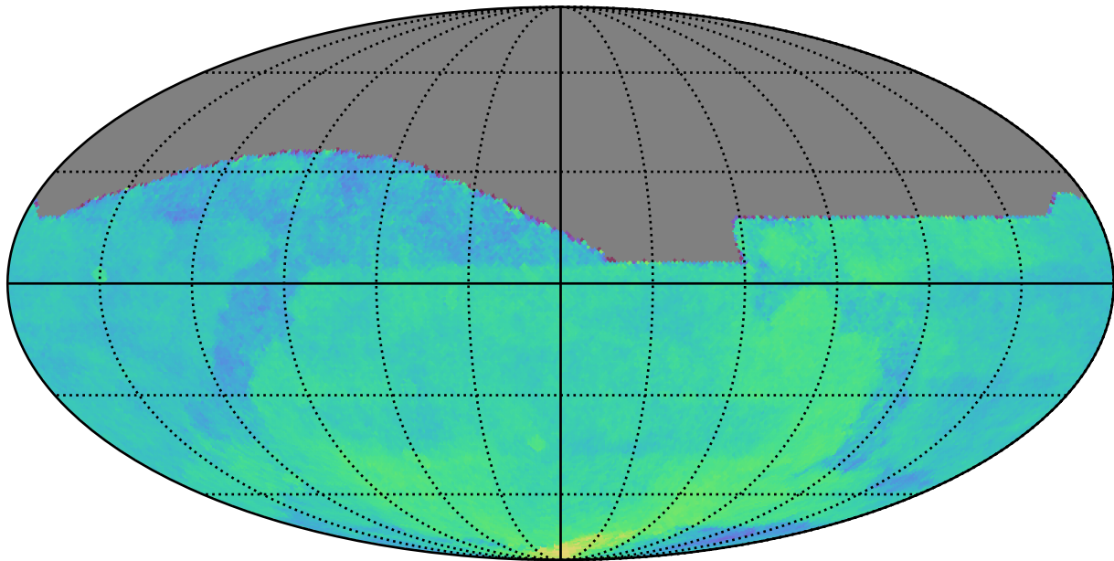
weather_cloudso4v3.4_10yrs All sky: Parallax Coverage @ 22.4
