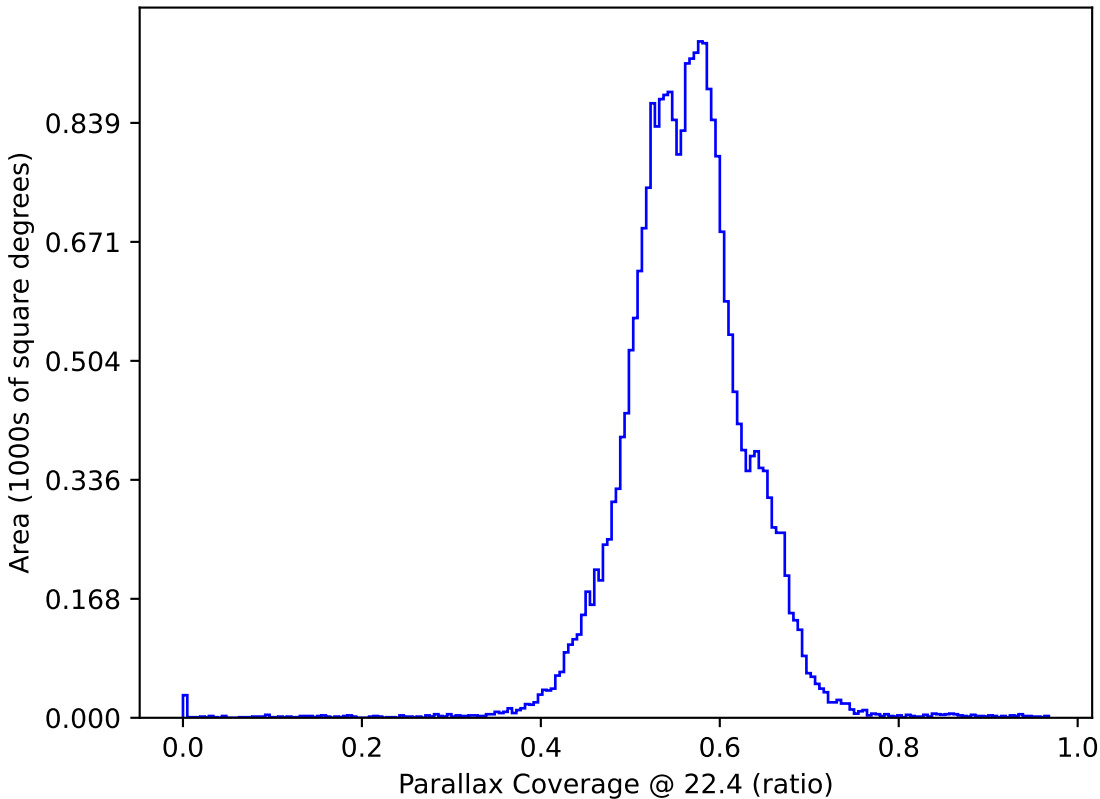
weather_cloudso4v3.4_10yrs All sky: Parallax Coverage @ 22.4
