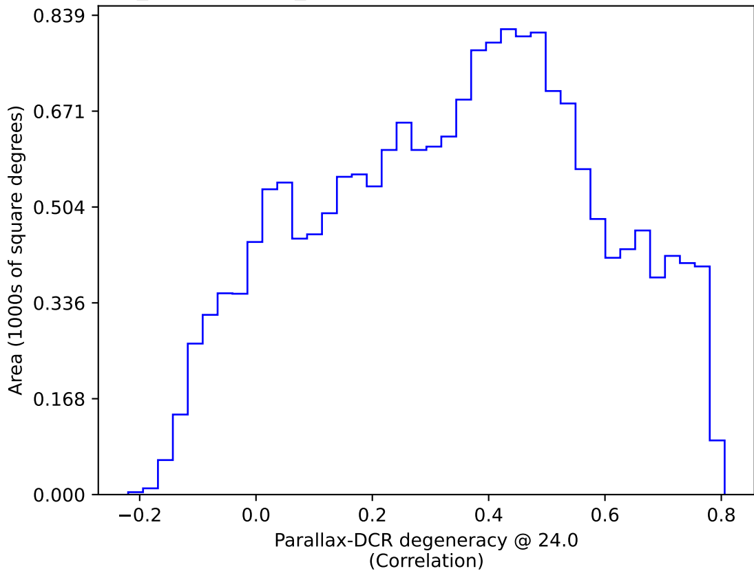
weather_cloudso4v3.4_10yrs WFD: Parallax-DCR degeneracy @ 24.0
