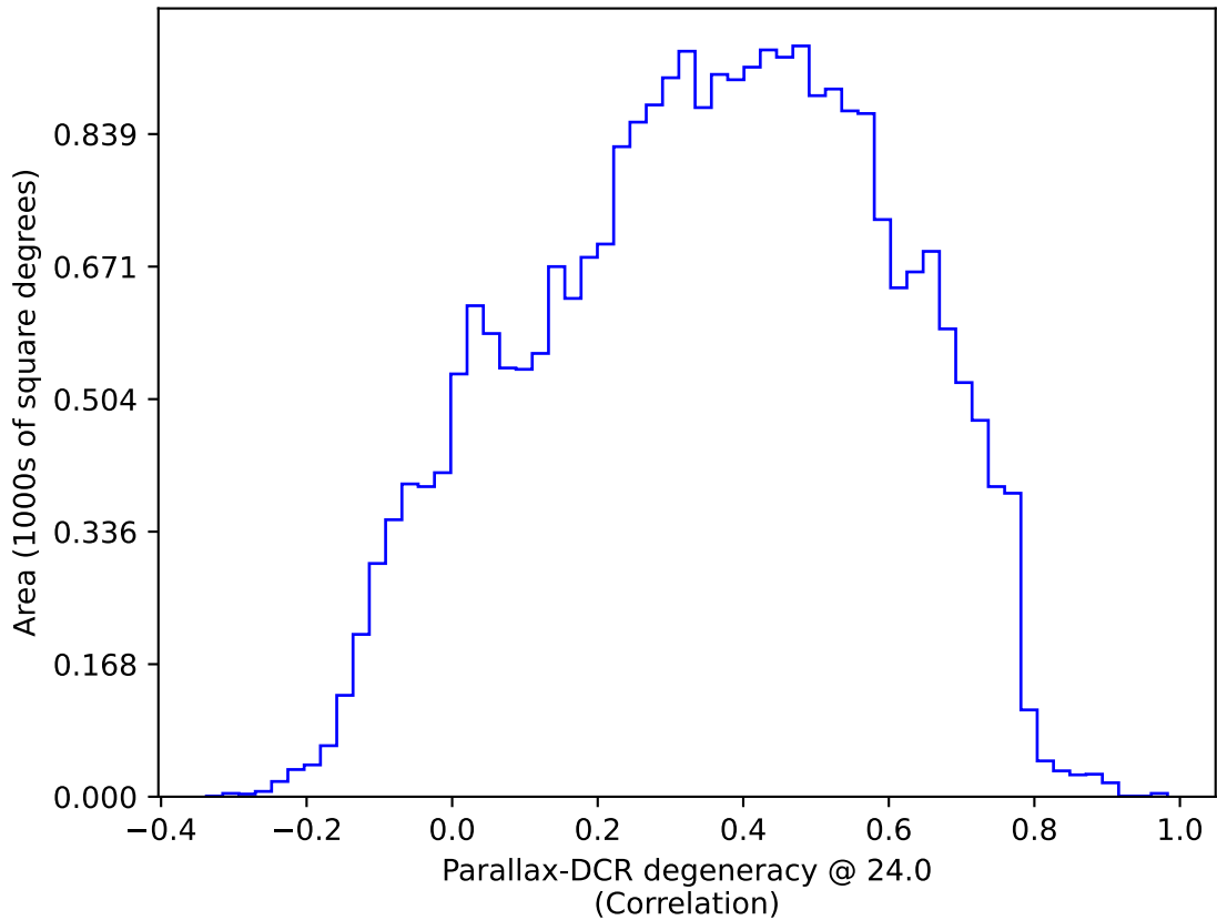
weather_cloudso4v3.4_10yrs All sky: Parallax-DCR degeneracy @ 24.0
