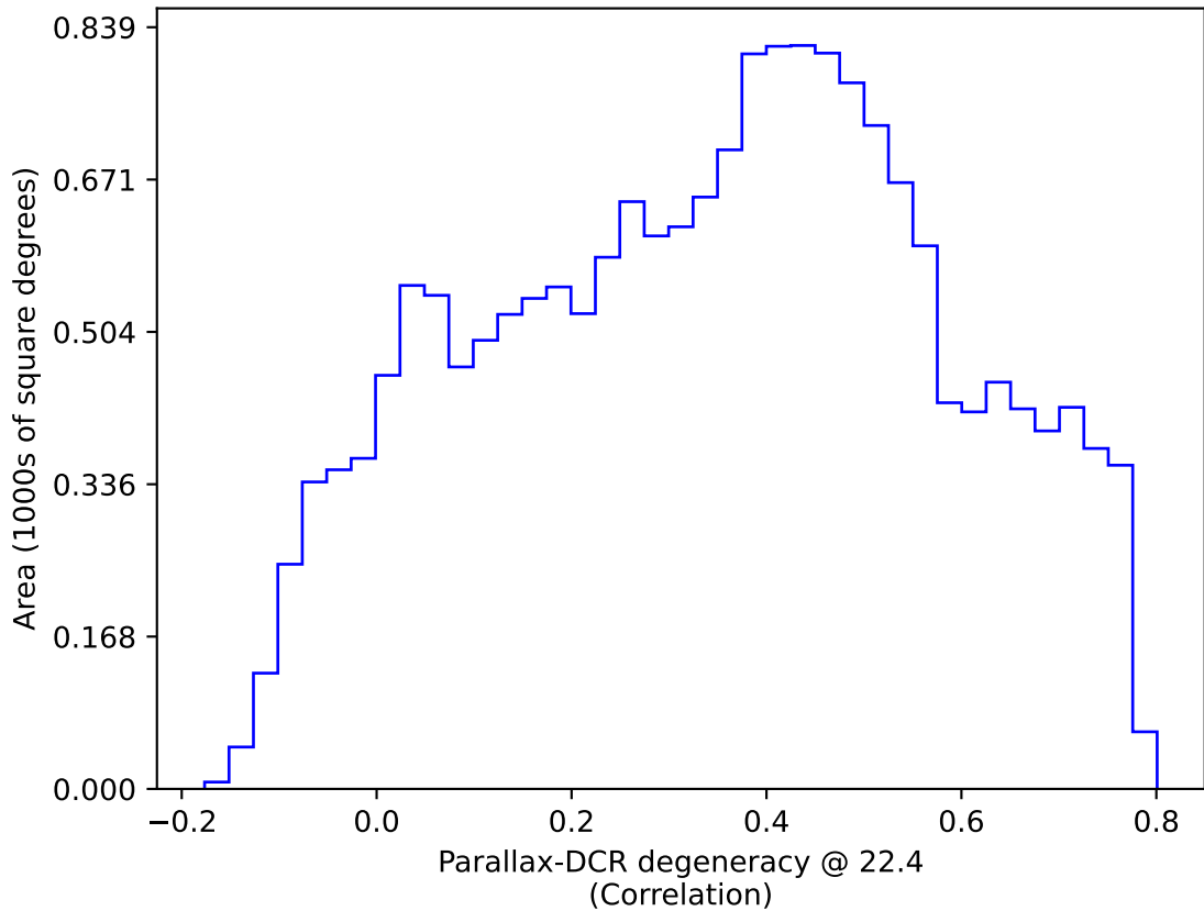
weather_cloudso4v3.4_10yrs WFD: Parallax-DCR degeneracy @ 22.4
