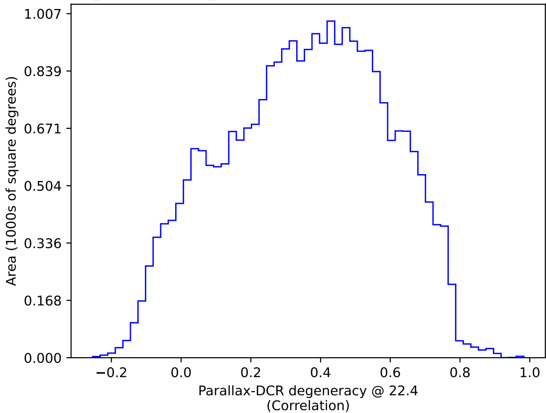
weather_cloudso4v3.4_10yrs All sky: Parallax-DCR degeneracy @ 22.4
