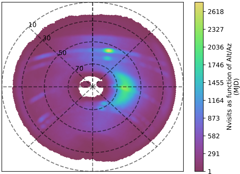
weather_cloudso4v3.4_10yrs z band: Nvisits as function of Alt/Az
