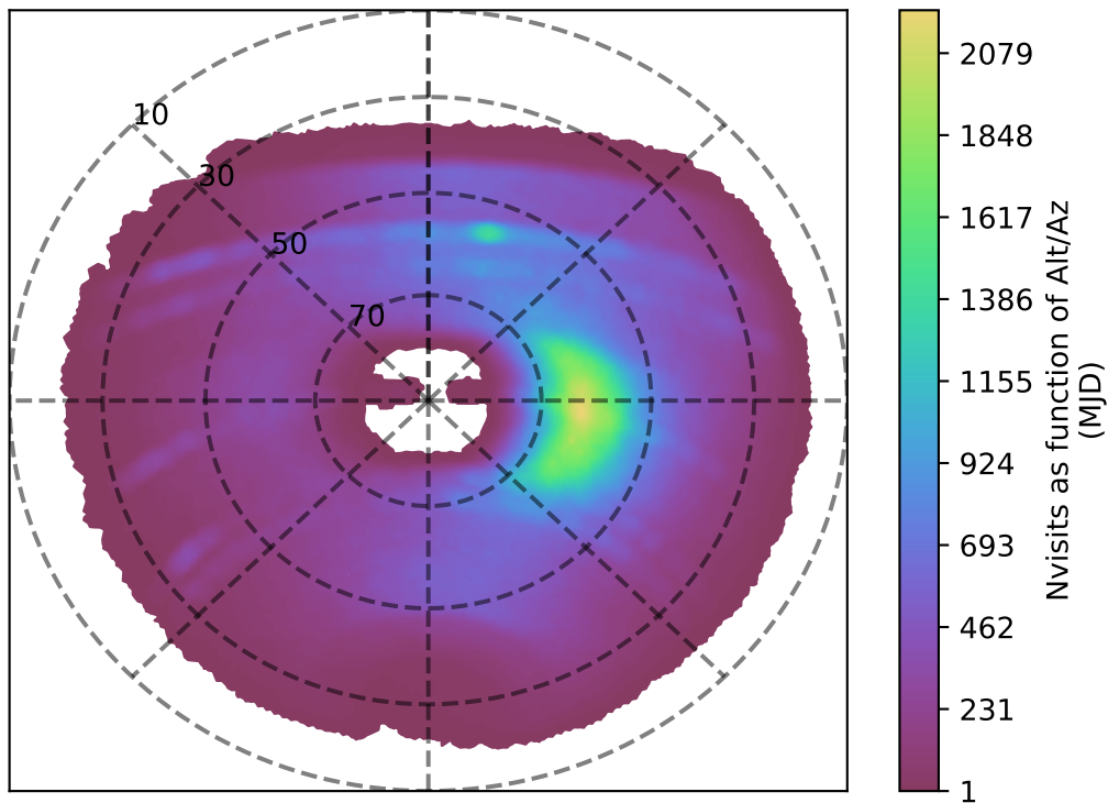
weather_cloudso4v3.4_10yrs y band: Nvisits as function of Alt/Az
